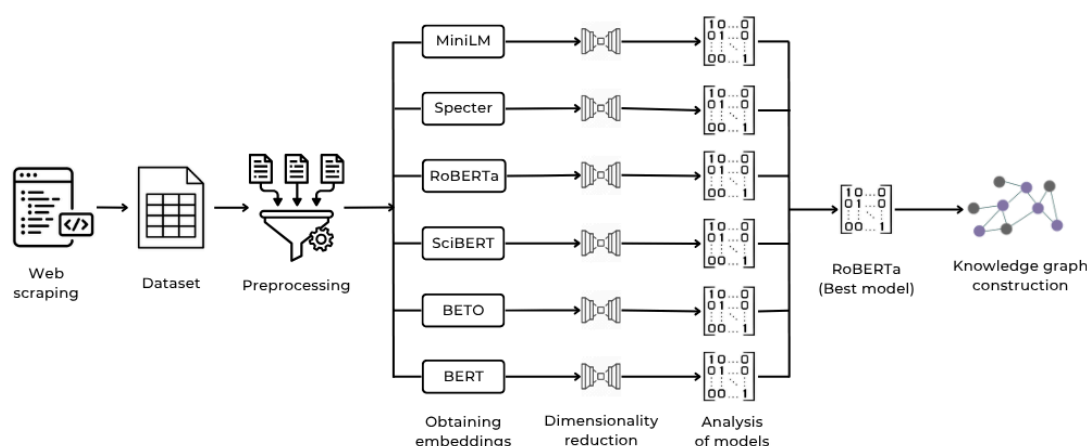
Figure 1: Semantic pipeline for similarity analysis in academic works
