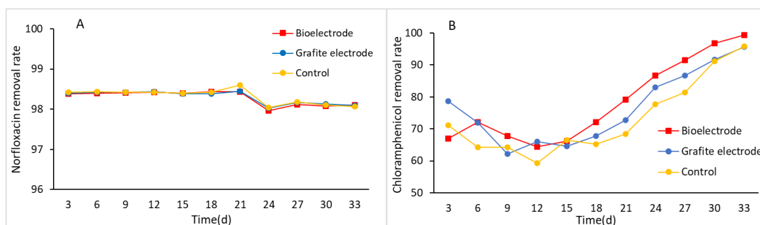
Figure 1. Removal of Norfloxacin (A) and Chloramphenicol (B) throughout the experiment for the two electrodes and the control group.
